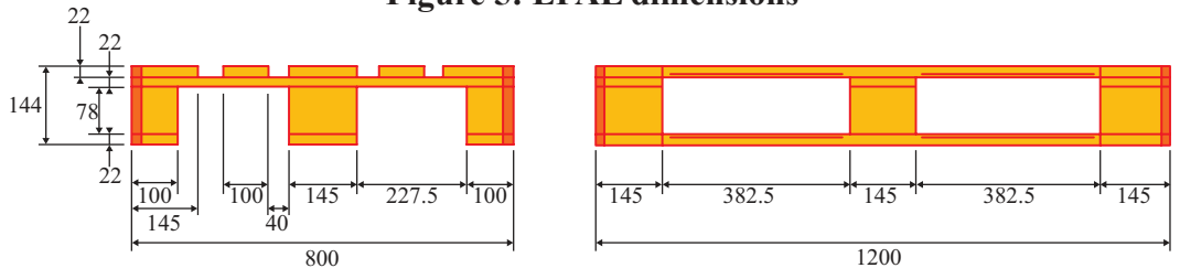
Figure 5: EPAL dimensions
